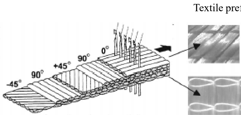
Figure 7 Multiaxial weft inserted warp knit (MWK).
