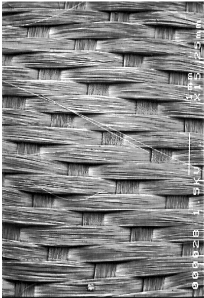
8 harness satin
