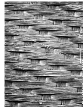
8 Harness satin
