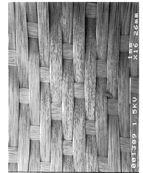
8 Harness satin
