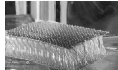
Figure 41 Sandwich-fabric preform.
