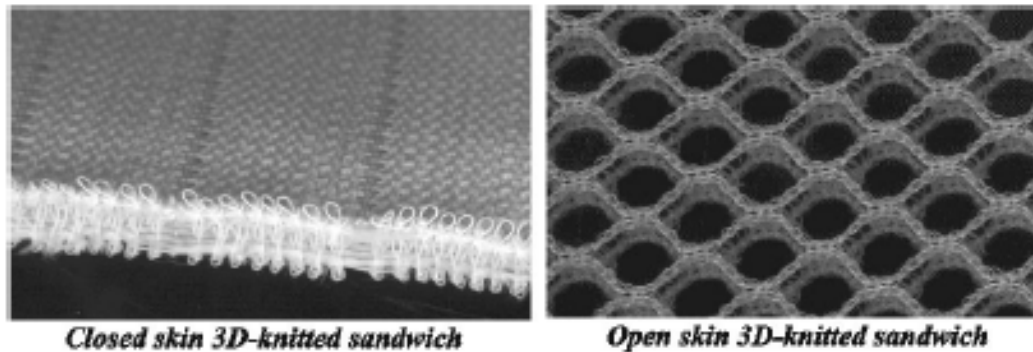
Figure 47 Comparison of a closed-skin 3-D knit with an open 3-D knit. The closed-skin knit is very similar to a 3-D weave.
