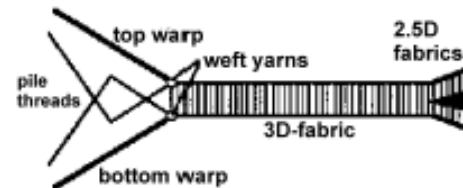
Figure 40 Schematic of velvet weave
