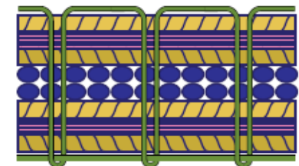
Knitted/stitched
