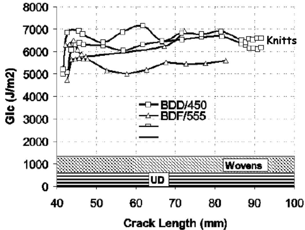
Mode I fracture toughness of glass/epoxy composites tested in the wale direction
