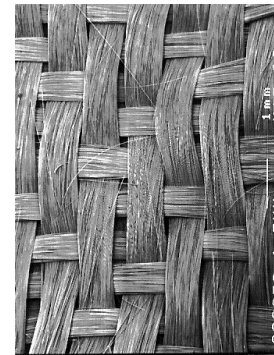
4 Harness satin
